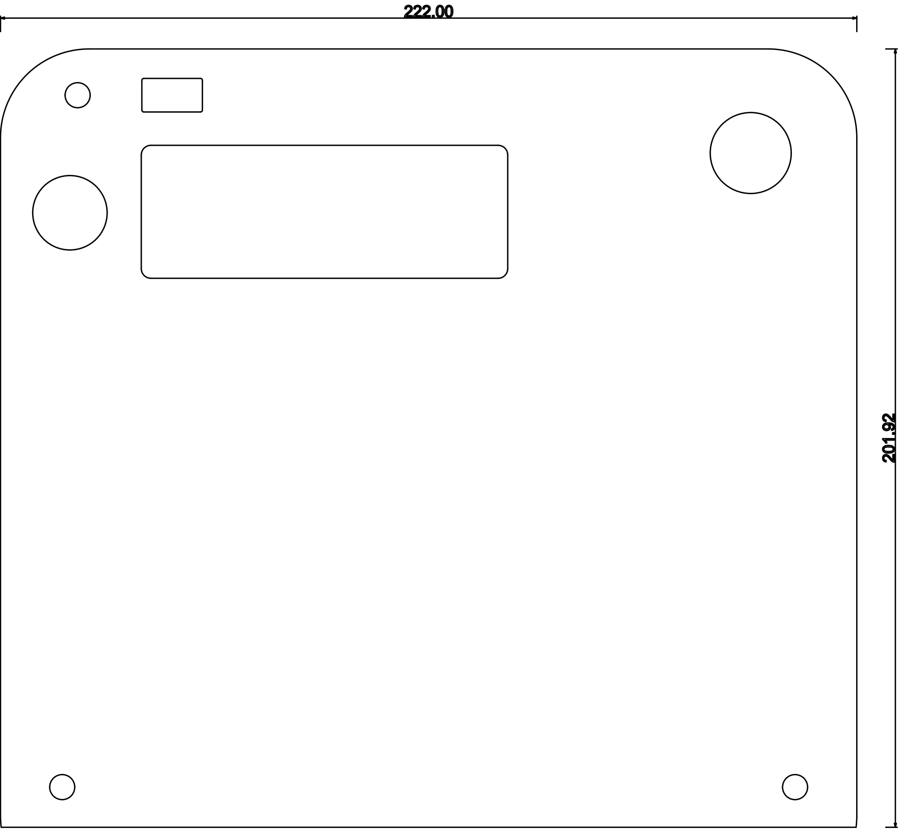
FRONT PANEL
